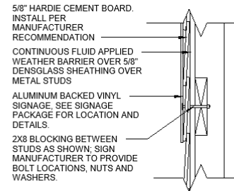
12 VINYL SIGNAGE BLOCKING @ HARDIE 1 1/2" = 1'-0"
