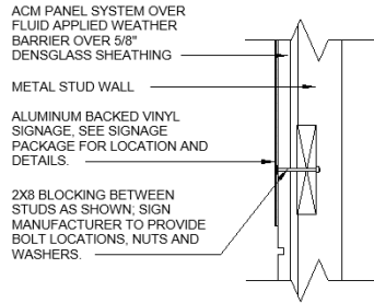
4 VINYL SIGNAGE BLOCKING @ ACM 1 1/2" = 1'-0"
